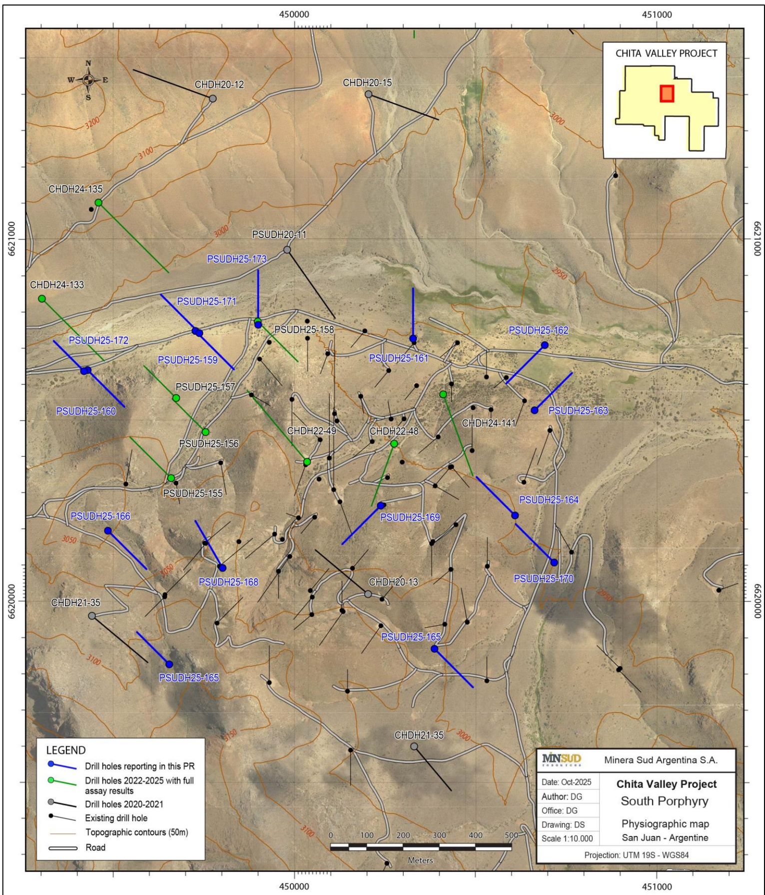
Map 1. Location of PSU in-fill drillholes
